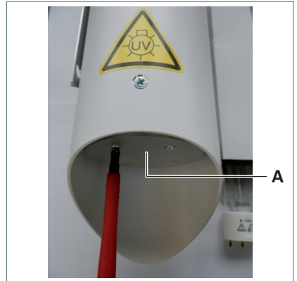
Fig. 1: Remove lamp cover.
