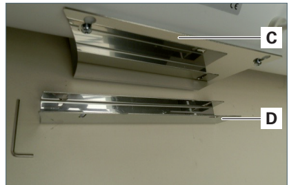
Fig. 5: Loosen the screws.
